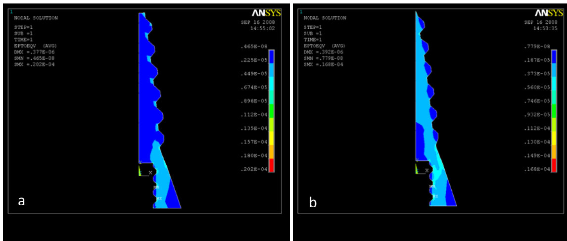
Figure 14. von Mises strain distribution in conic type 4 with 0.12 gradient from .465 \times 10^{-8} to .202 \times 10^{-4} Pa; the highest max stress is generated in this type (a); and conic type 5 with 0.16 gradient from 0.779 \times 10^{-8} to 0.168 \times 10^{-4} Pa (b).
