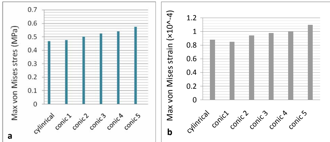
Figure 10. Maximum von Mises stress (a) and strain (b) in all bones under 30 psi axial pressure.
