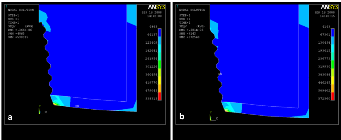
Figure 7. von Mises stress distribution in the conic type 4 with 0.12 gradient from 4865 Pa to 538315 Pa (a) and conic type 5 with 0.16 gradient from 4143 Pa to 572560 Pa; highest max stress is generated in this type (b).
