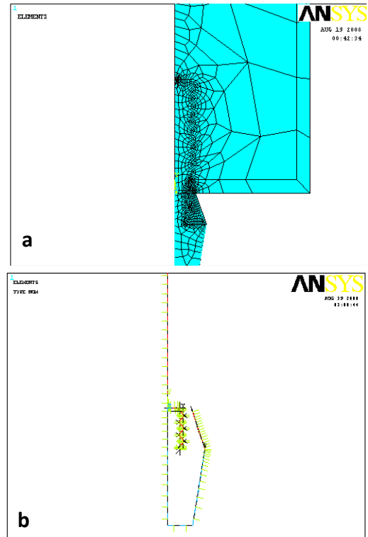
Figure 4. Meshing with plane 83 elements (a) and using contact element between implant and abutment (b).
