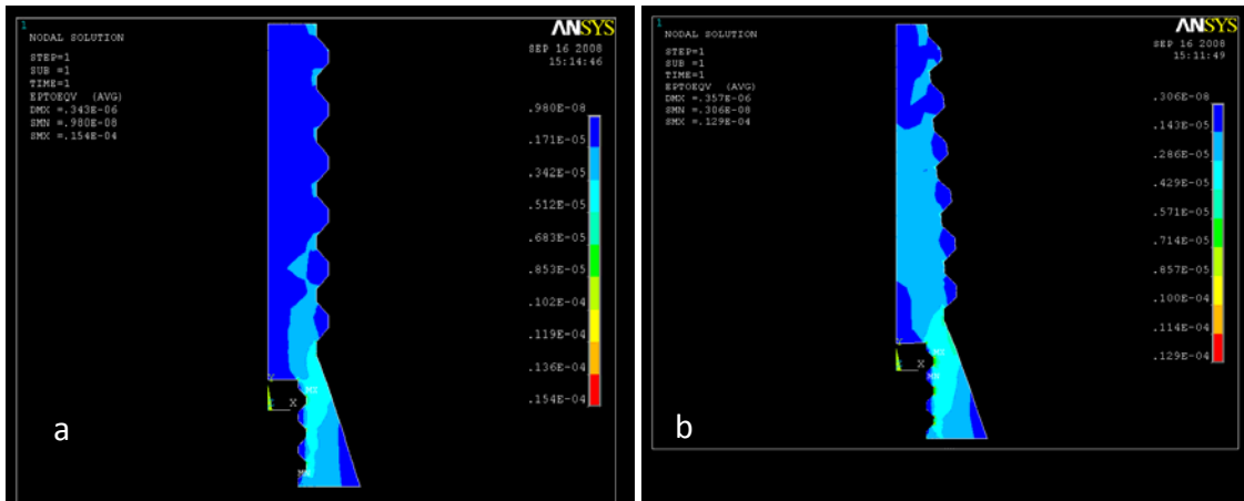
Figure 13. von Mises strain distribution in the cylindrical type .98 \times 10^{-8} to .154 \times 10^{-4} Pa (a) and conic type 2 with 0.06 gradient from .306 \times 10^{-8} to .129 \times 10^{-4} Pa; lowest maximum strain is generated in this type (b).
