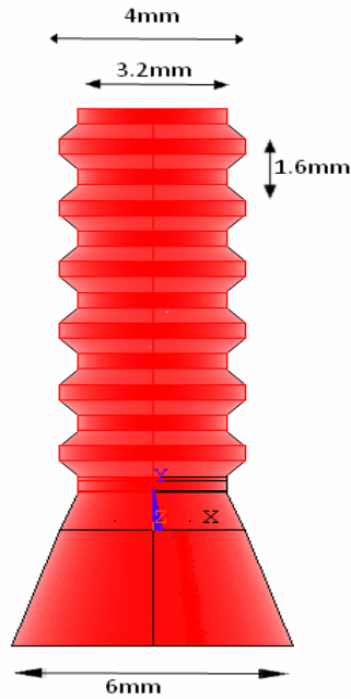
Figure 3. Implant dimension.
