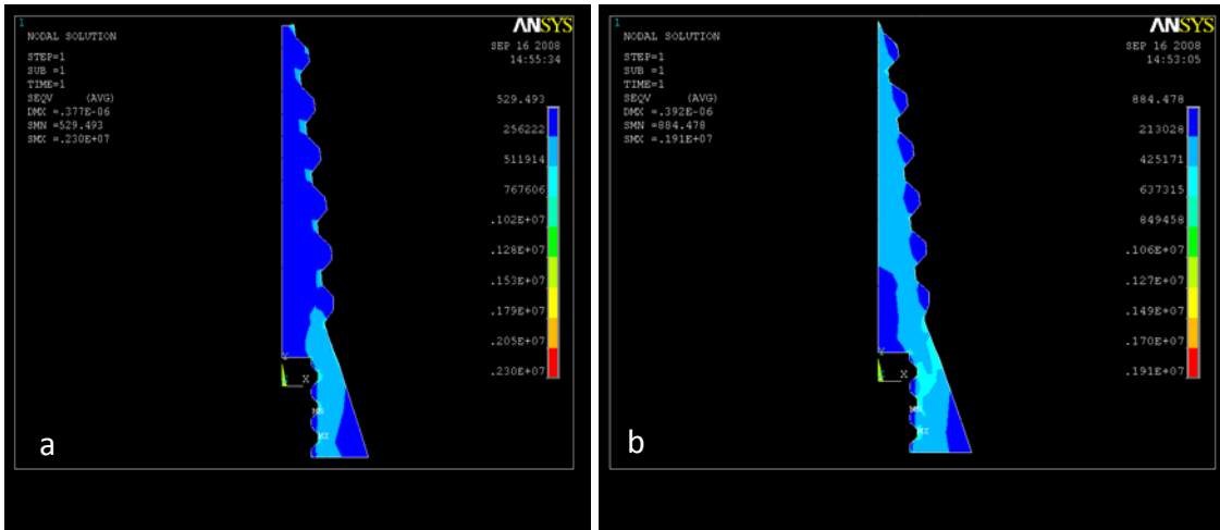
Figure 12. von Mises stress distribution in the conic type 4 with 0.12 gradient from 529.5 to .23 \times 10^7 Pa, the highest max stress is generated at this type (a) and conic type 5 with 0.06 gradient from 884 to .191 \times 10^7 Pa (b).
