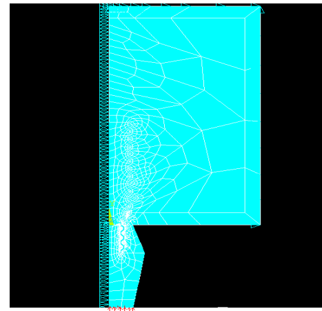
Figure 5. Boundary condition symmetry on left boulder of model and using 30 psi on lower edge of abutment.
