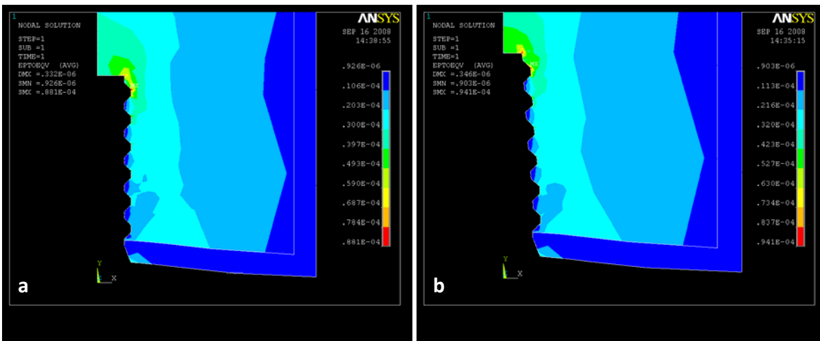
Figure 8. von Mises strain distribution in the cylindrical from 0.926 \times 10^{-6} to 0.881 \times 10^{-4} Pa (a) and conic type 2 with 0.06 gradient from 0.903 \times 10^{-6} to 0.941 \times 10^{-4} Pa (b).
