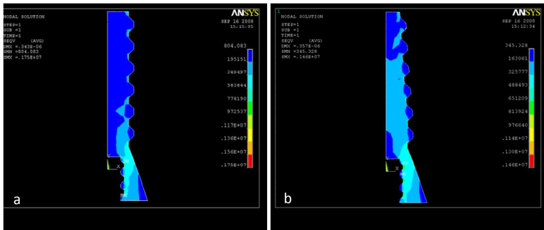
Figure 11. von Mises stress distribution in the cylindrical type from 804 to .175 \times 10^7 Pa (a) and conic type 2 with 0.06 gradient from 345 to .146 \times 10^7 Pa; lowest maximum stress is generated in this type (b).
