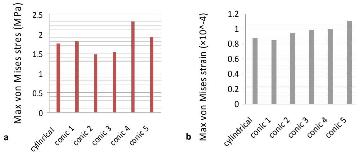
Figure 15. Maximum von mises stress (a) and strain (b) in all types of implants under 30 psi axial pressure.
